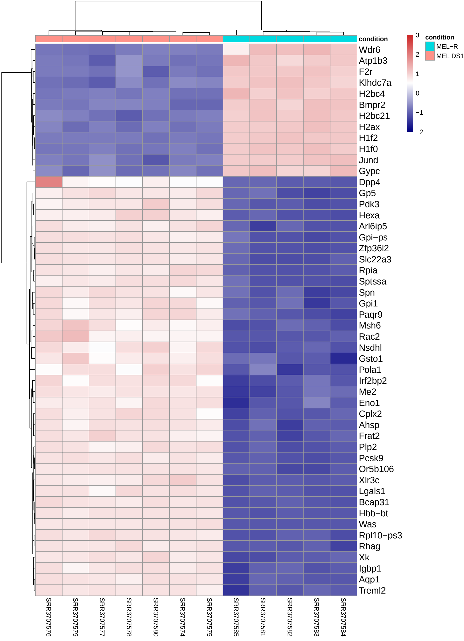
Salmon – Replication Fig 1B: Top 50 Genes.
